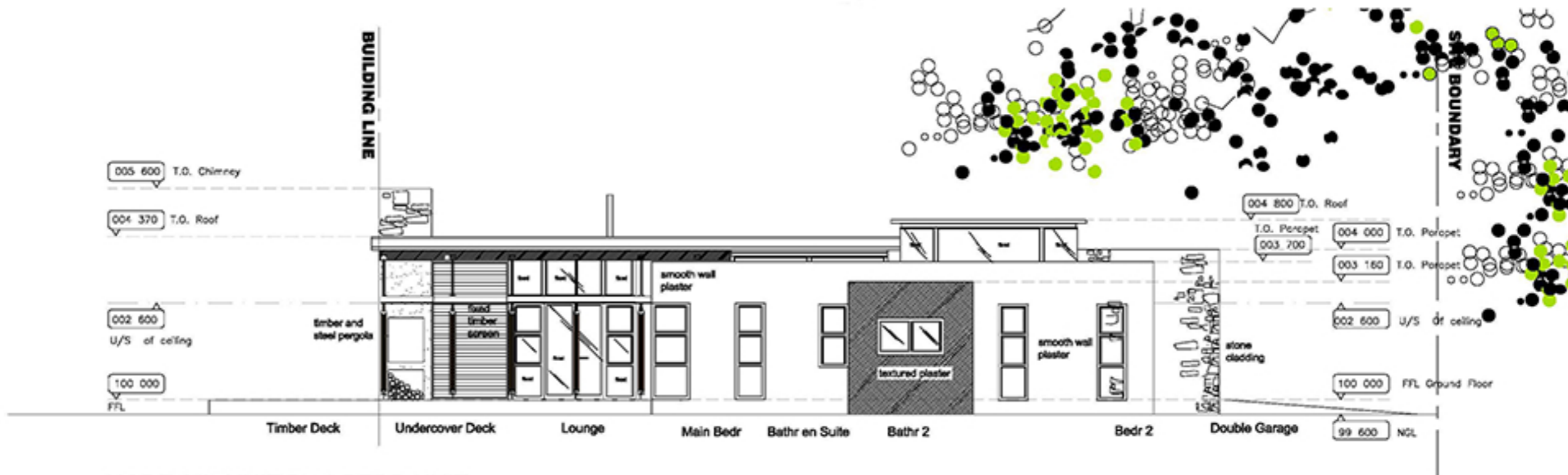
NODE 2/3: UNIT D : 3 BEDR UNIT North East Elevation
