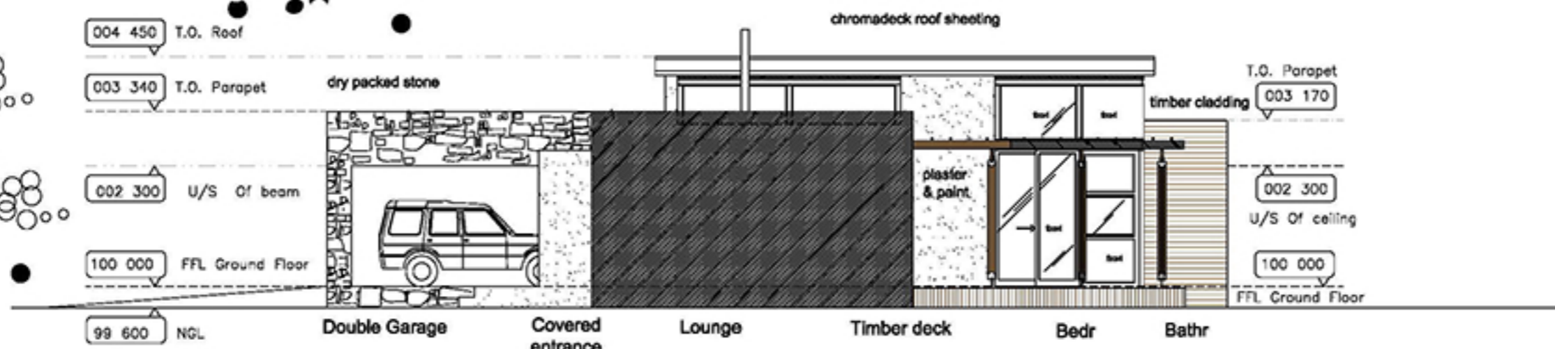
NODE 1: UNIT A: STUDIO UNIT East Elevation
